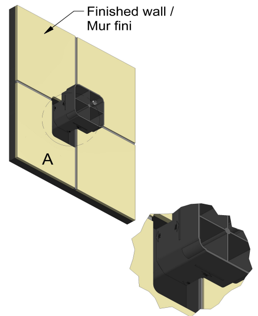
DETAIL A
